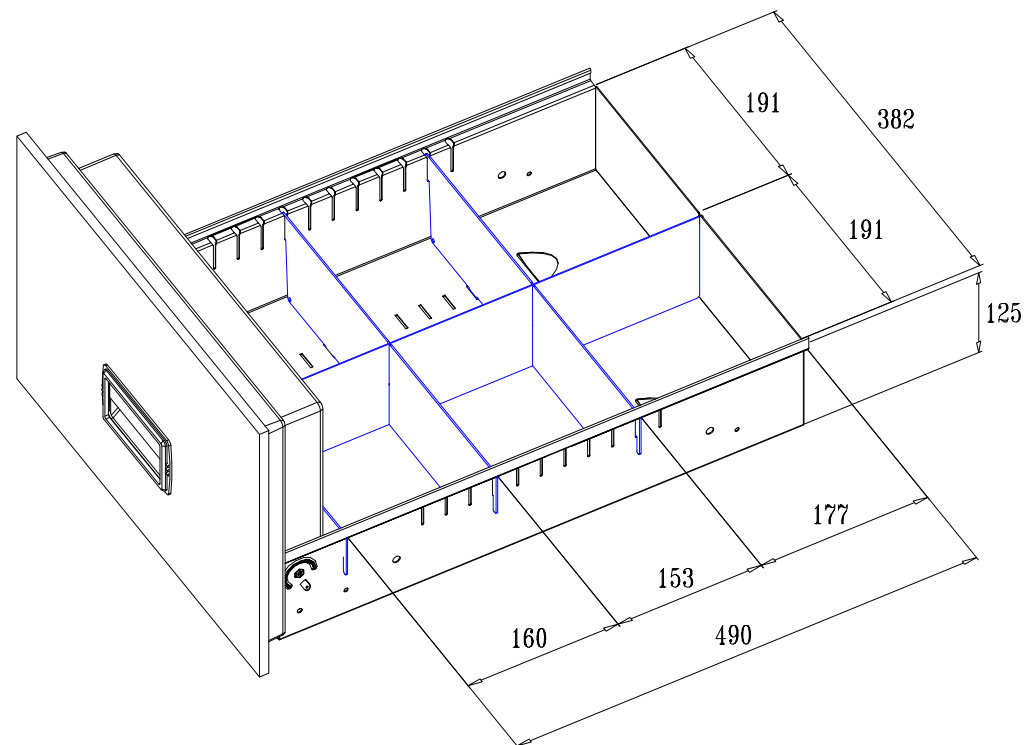
Drawer
